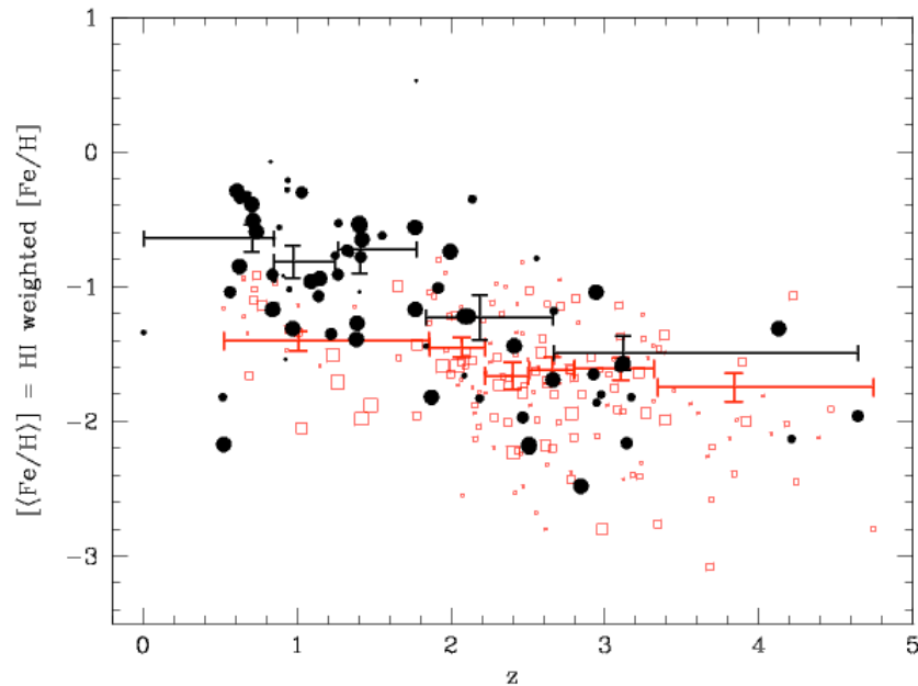
DLAs (red) and sub-DLAs (black)
